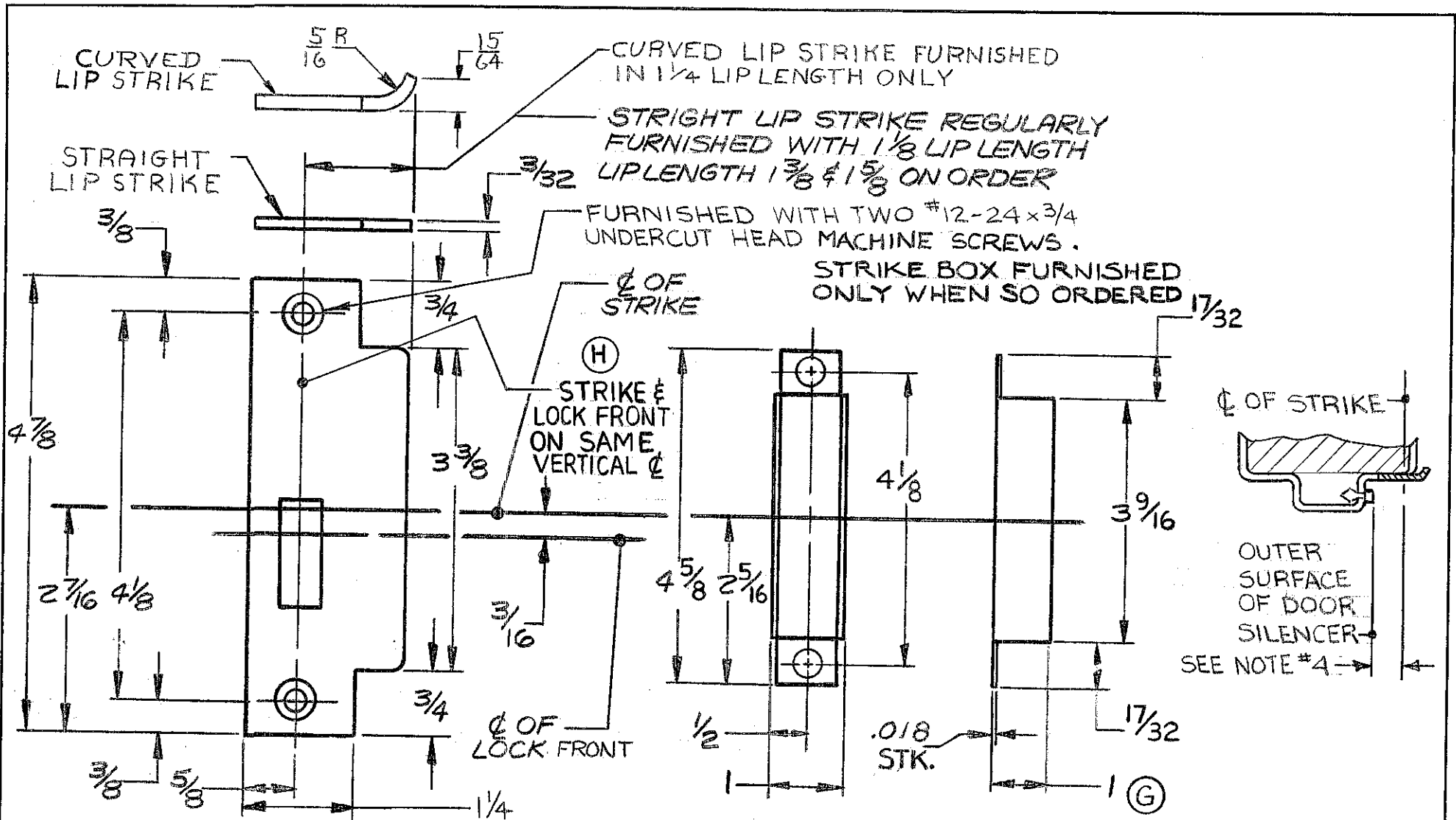
DETAIL OF STRIKE BOX
